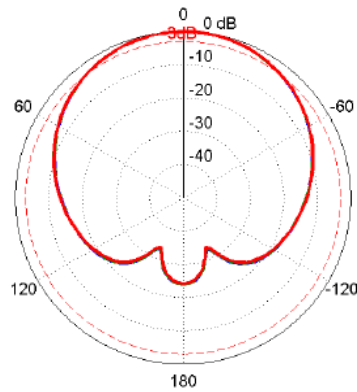
YZ Plane: 1561–1602 MHz
