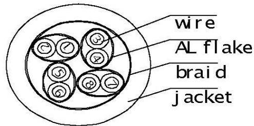
CAT.6 PIMF SHIELDED VOIP Patch Cable STRUCTURE
