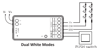
2 in 1 LED Controller (FUT035S+)
