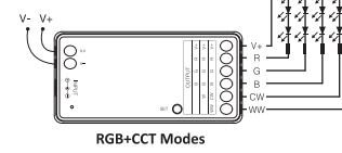
3 in 1 LED Controller (FUT037S+)
