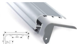
End cap with hole End cap without hole Aluminium profile PMMA opal milky cover PMMA smoke clear cover PMMA clear cover PC diffused cover
