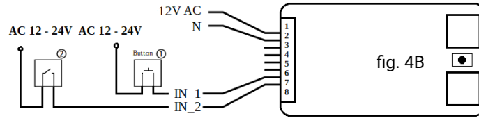
Wiring of buttons and switches
