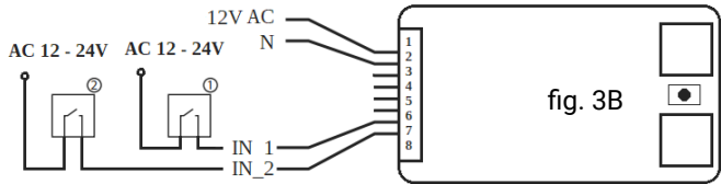
Wiring of binary sensor(Reed Ampule)
