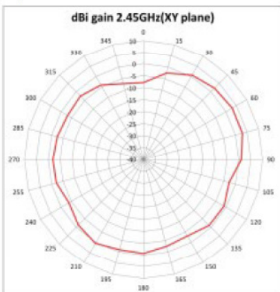
2,4-GHz-Antenne
