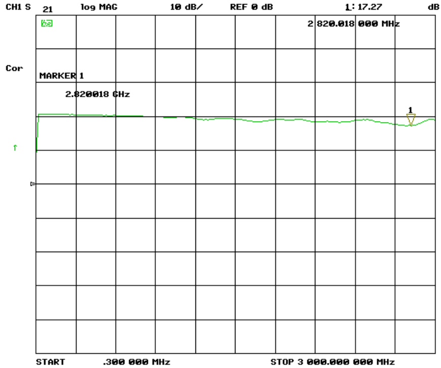
Picture 13 – TBWA2/20dB, gain, 300 kHz – 3 GHz, lin.
